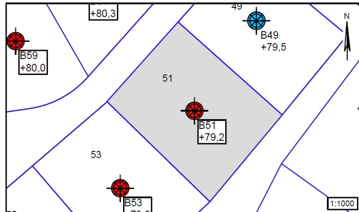
Figur 1 – Situationsplan 1:1000, Parcel nr. 51
